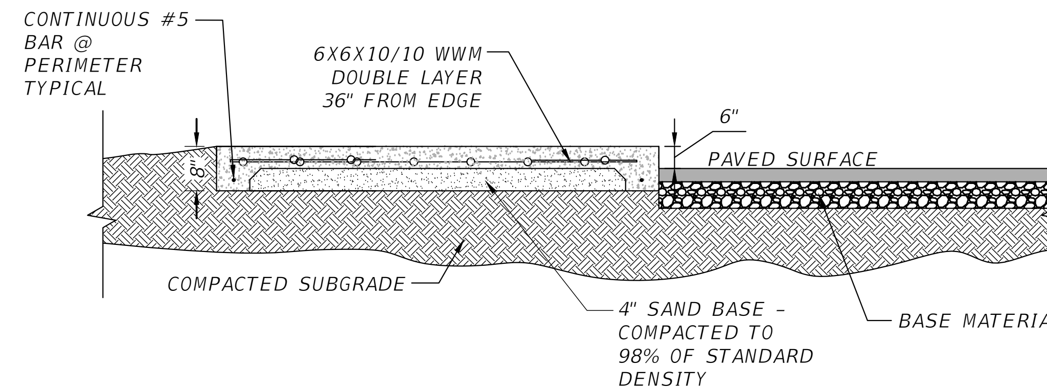
SECTION VIEW
