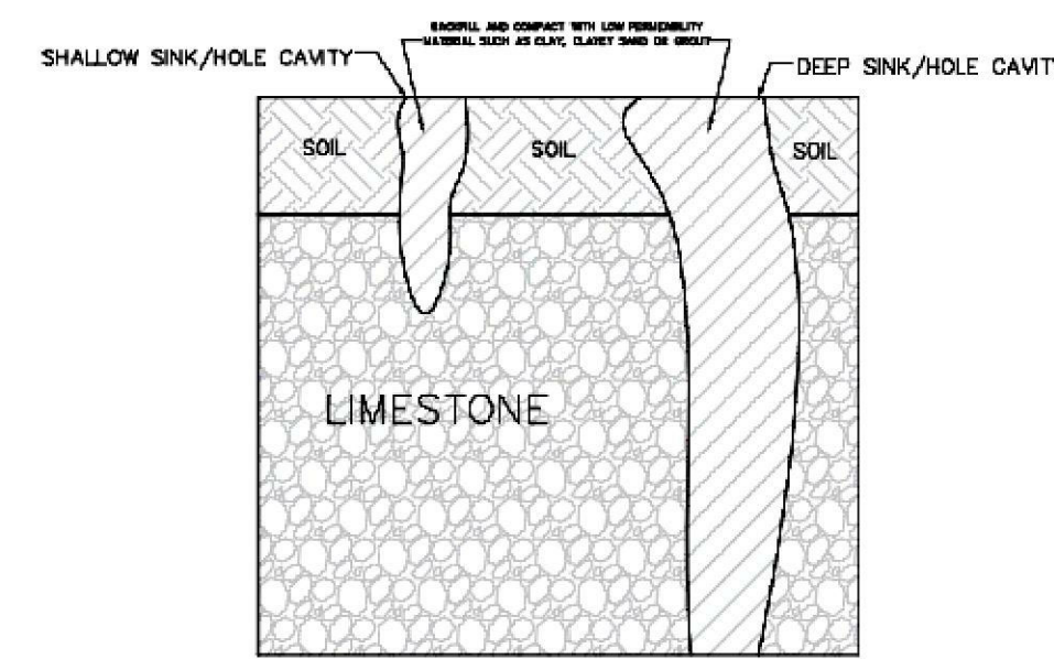
SHALLOW & DEEP SINK HOLE/CAVITY REPAIR & MAINTENANCE DETAIL CONTACT GEOTECHNICAL ENGINEER FOR FURTHER EVALUATION & ADDITIONAL REMEDIATION MEASURES IF NEEDED
